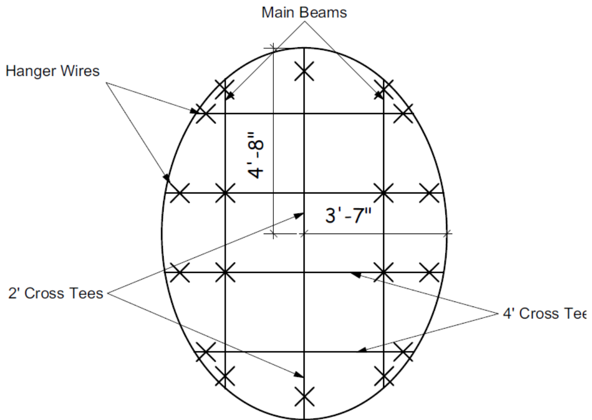
Figure 31 - Hanger Wire Layout
