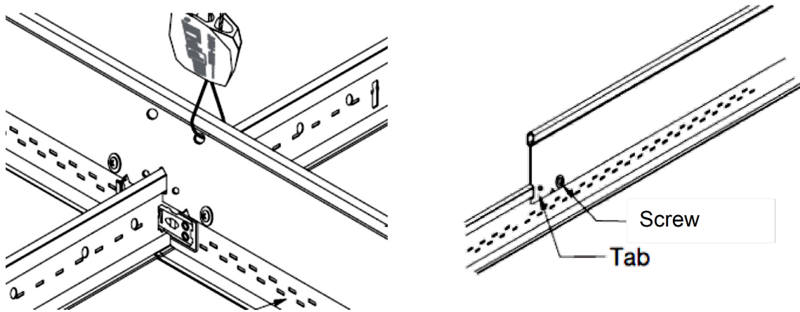
Figure 19 - Strong back Connection to Cross Tees Figure 20 – Setting Cross Tee Elevation
