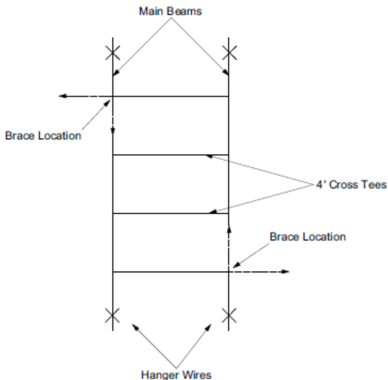
Figure 32 - Diagonal Brace Locations
