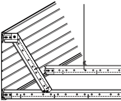
Figure 36 - Braced Perimeter Trim
