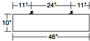
Figure 43 - 10" Blades
