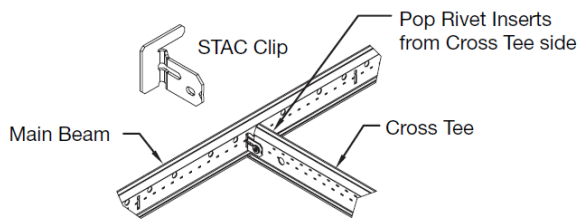
Figure 17 - STAC Clip Placement and Attachment
